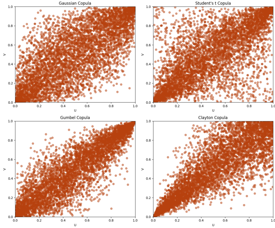
FIGURE 5: Different copulas
