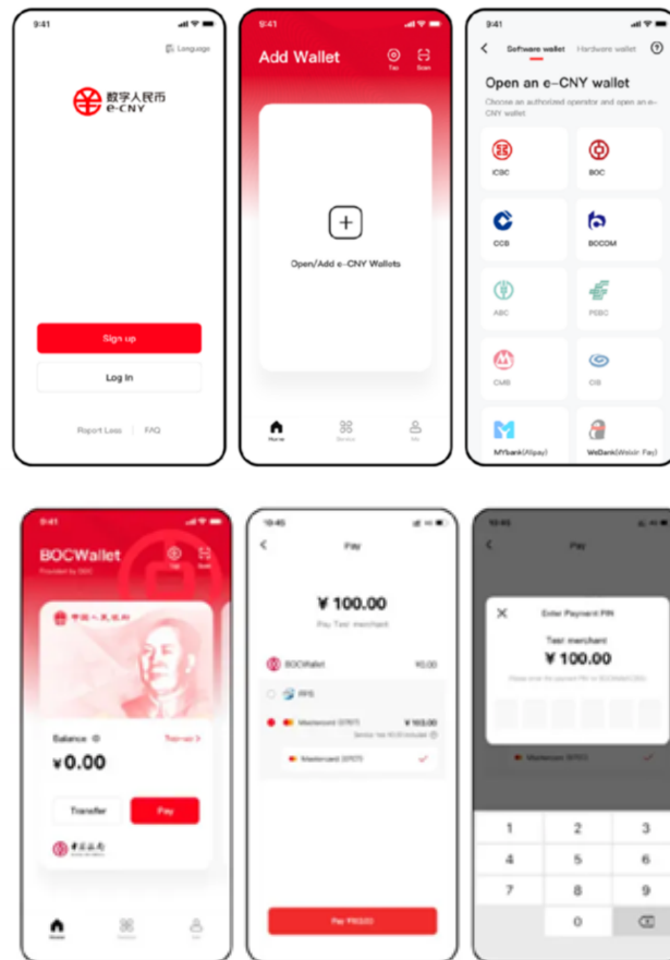
FIGURE 11: e-CNY APP [36]
