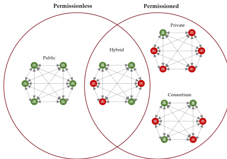
FIGURE 4: DLTs Architectures.
